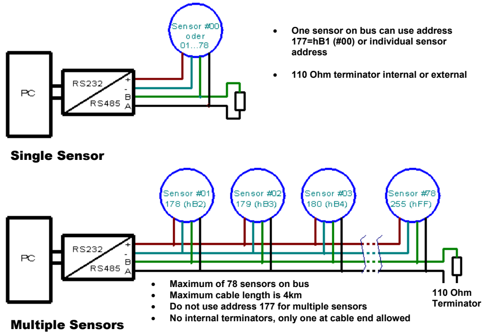
Figure 3: NG360 Sensor Connection to RS485 Bus
