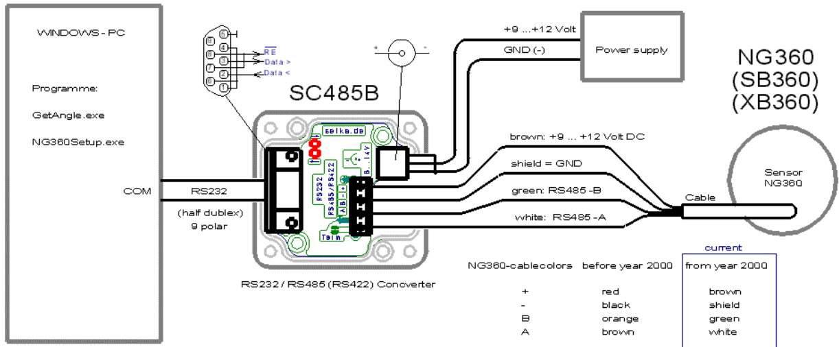
Figure 2: Connection to RS232/RS485 converter (p/n SC485B)
