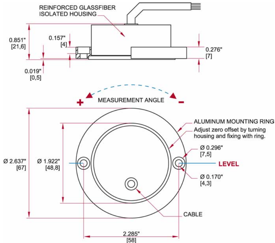
Figure 1: Dimensions and Mounting Position (inches [mm])
