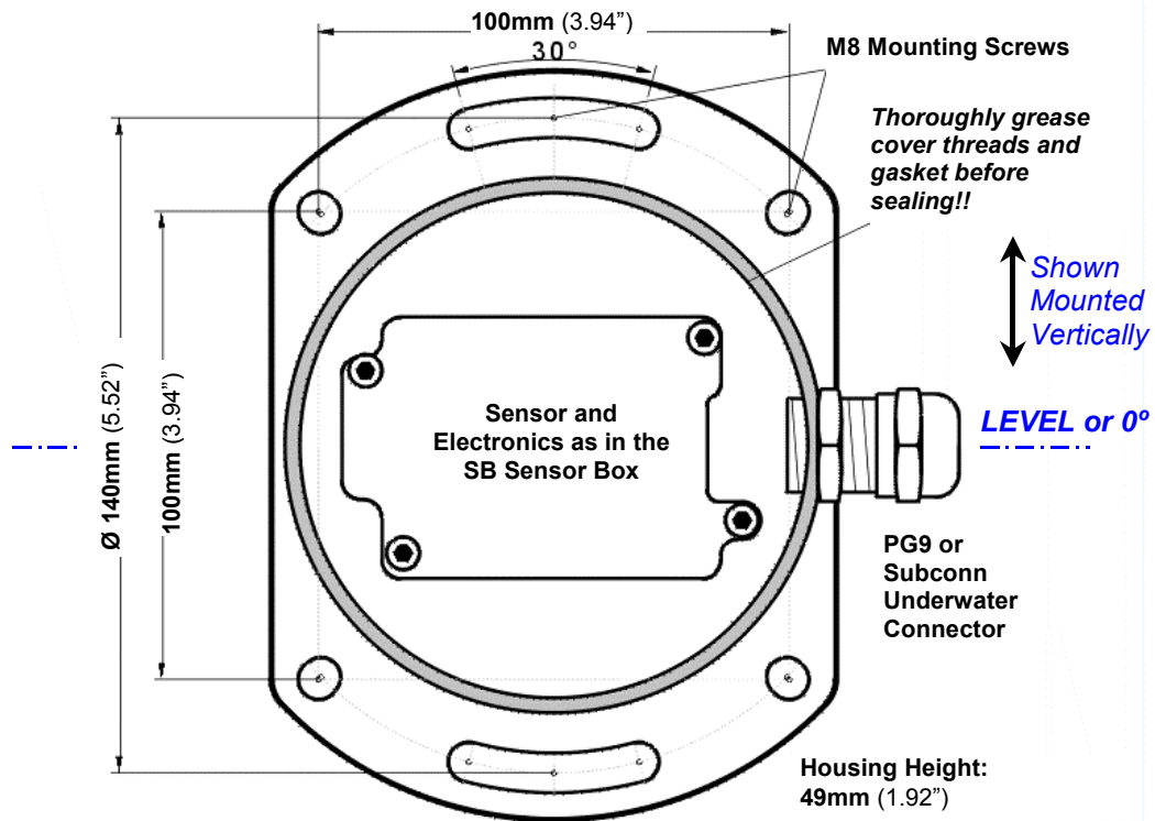
Figure 1: Dimensions and Mounting Position (inches [mm])
