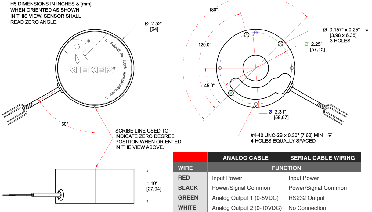
Figure 1: Dimensions and Wiring Connections
